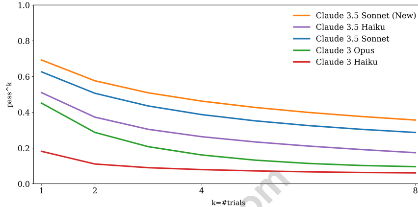
Figure 1 pass k for TAU-retail
