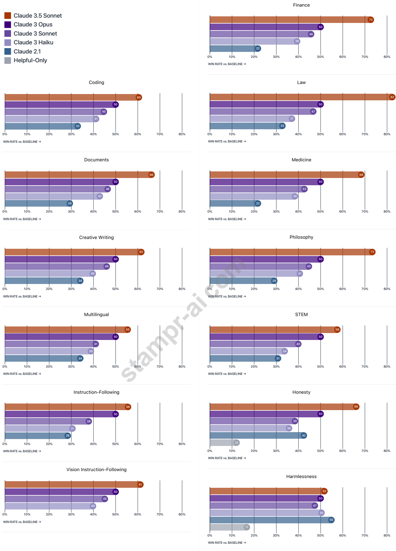
Figure 3 These plots show per-task human preference win rates for: common use cases (left), expert knowledge (top right), and adversarial scenarios (bottom right). Since Claude 3 Opus is the baseline model, it always has a 50% win rate. (It beats itself 50% of the time.)
