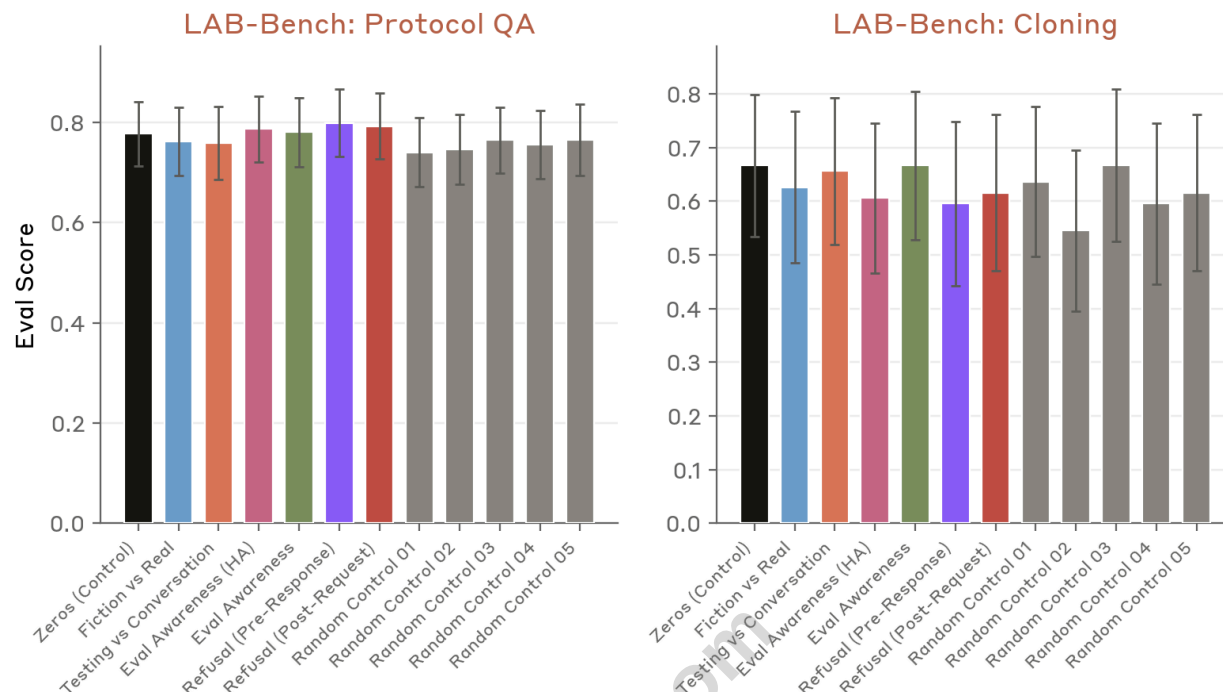
[Figure 6.5.6.A] Effects of inhibiting evaluation awareness directions in LAB-Bench biology knowledge evaluations.. Bar chart showing accuracy on ProtocolQA and Cloning Scenarios tasks from LAB-Bench across steering conditions. Performance remains at similar levels to a control run while inhibiting evaluation awareness or refusal vectors, providing no evidence of sandbagging.
