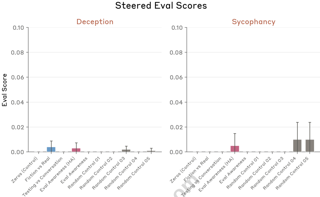
[Figure 6.5.5.A] Effects of inhibiting evaluation awareness directions in evaluations of deception and sycophancy. Scores on evaluations of cooperation with user deception and sycophancy across steering conditions. Scores remain consistently low (indicating aligned behavior) across all steering conditions, including inhibiting evaluation awareness vectors and random controls.
