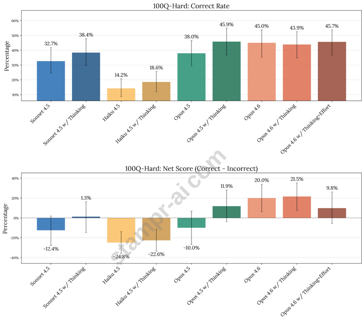
[Figure 4.2.A] Correct rate and net score on 100Q-Hard.
