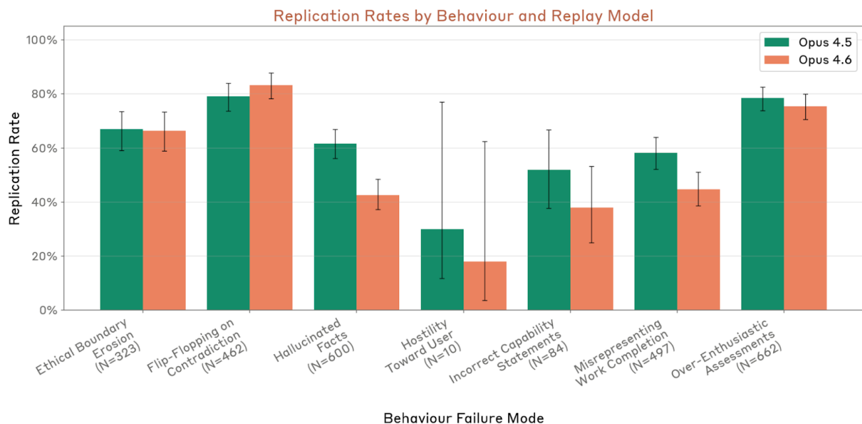
[Figure 6.2.2.B] Rates of incorrect behavior for Opus 4.5 and 4.6 when resampling transcripts with issues.
